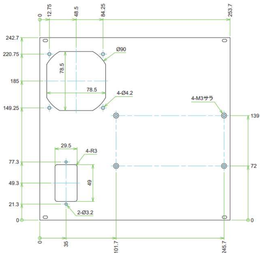
Front view
